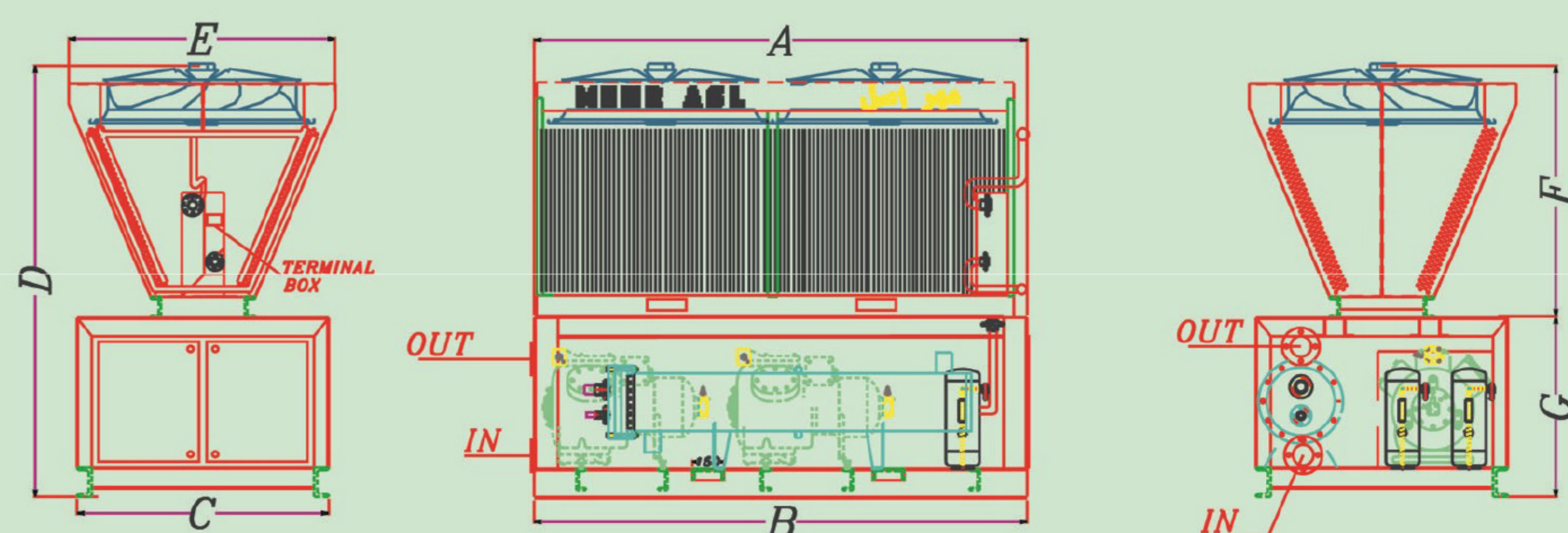
7LC***40&7LC***50&7LC***60 DIMENTION
