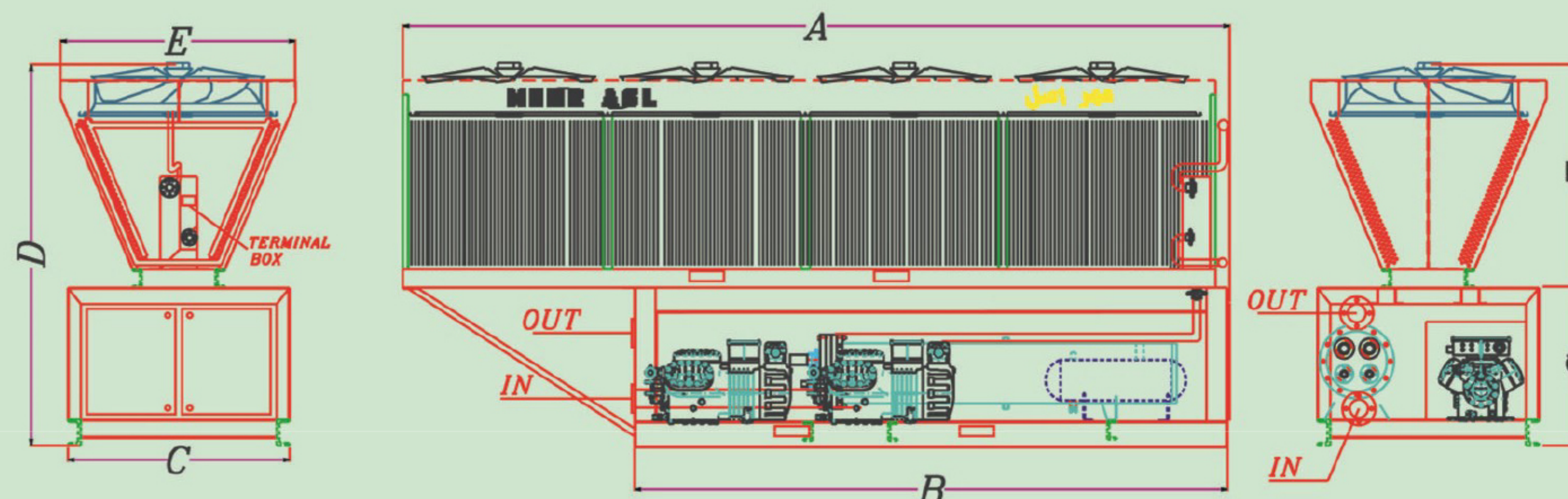
7LC***70&7LC***80&7LC***90&7LC***100&7LC***110 MODELS DIMENTION
