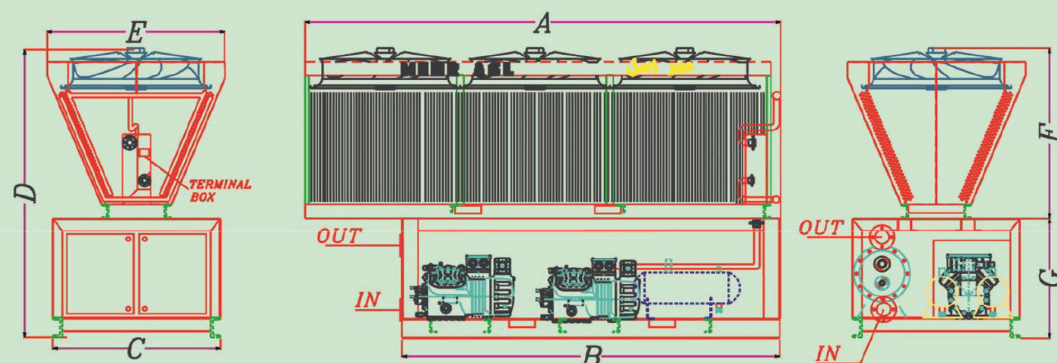
7LC***50&7LC***60&7LC***70&7LC***80 DIMENTION
